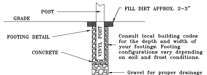
FIGURE 6.4 POST HOLE DETAIL
