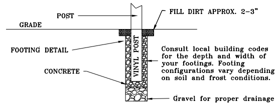
FIGURE 2.4 POST HOLE DETAIL
