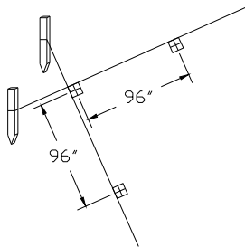
Figure 2.1 Mark the center for each post along the string line
