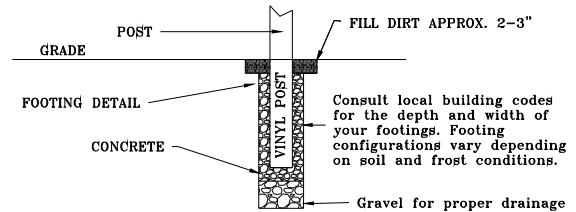
FIGURE 4.4 POST HOLE DETAIL
