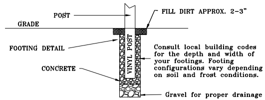
FIGURE 5.4 POST HOLE DETAIL
